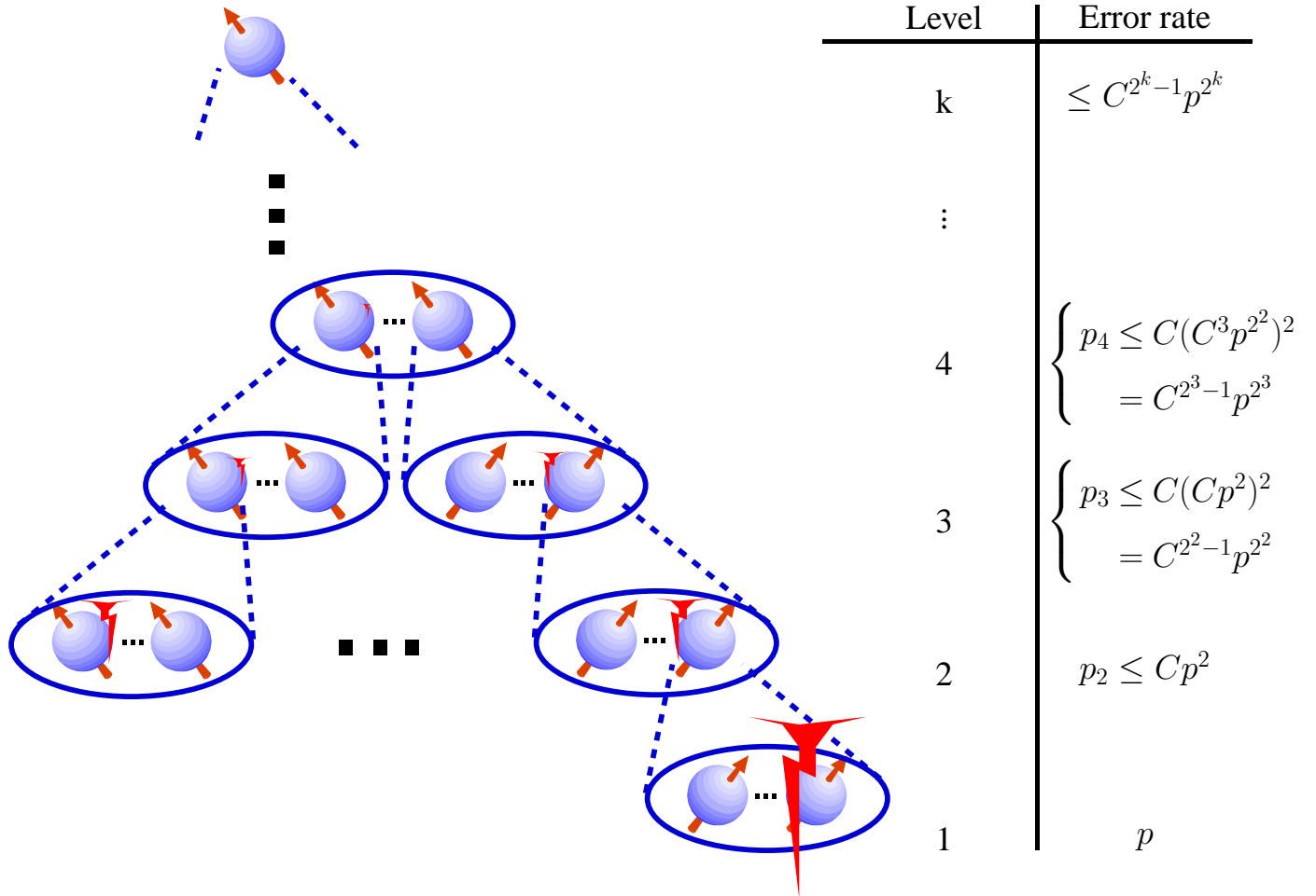
FIG. 9: Schematic representation of concatenation. The bottom level represents qubits realized more-or-less directly in a physical system. Each next level represents logical qubits defined by means of subsystems in terms of the previous level’s qubits. More efficient subsystems might represent multiple qubits in one code block rather than the one qubit per code block shown here.
