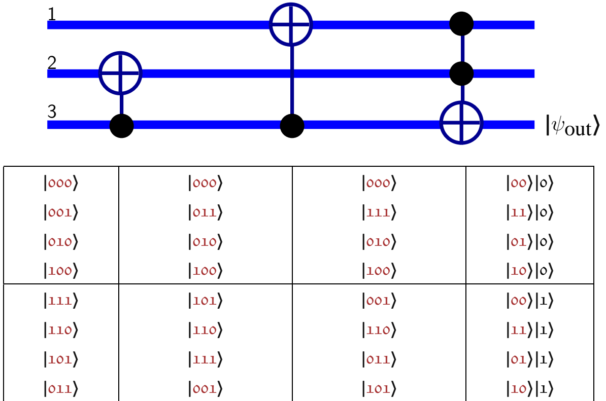
FIG. 5: Quantum network for majority logic decoding into the output qubit 3. The effect of the network on the basis states is shown, with the top half showing the states with majority 0. The decoded qubit is separated in the last step. The quantum network conventions are as explained in [16].
